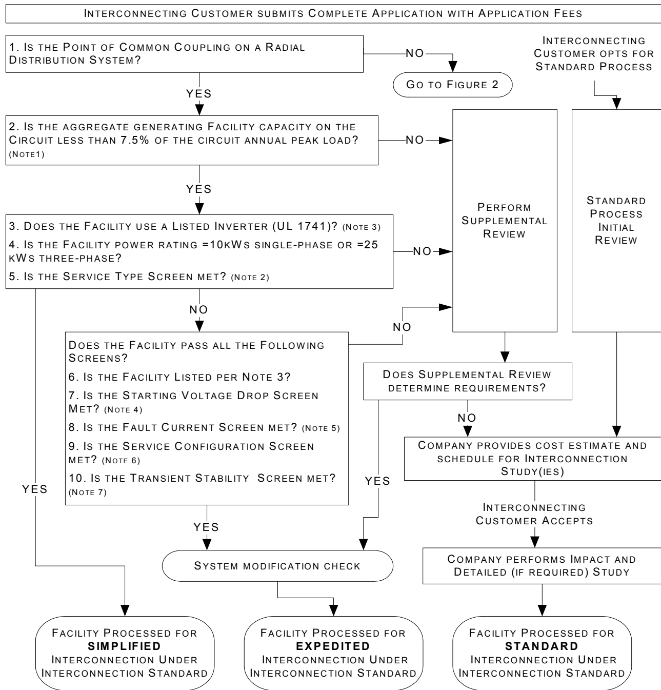
Figure 1 – Schematic of DG Interconnection Process
